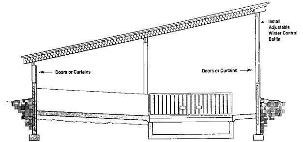
Figure 6. Single slope roof, partial slats building.
