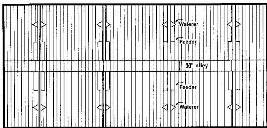
Figure 7. Totally slotted floor building with a center alley.
