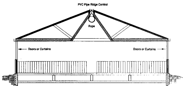
Figure 9. Continuous, sloped center chimney building.
